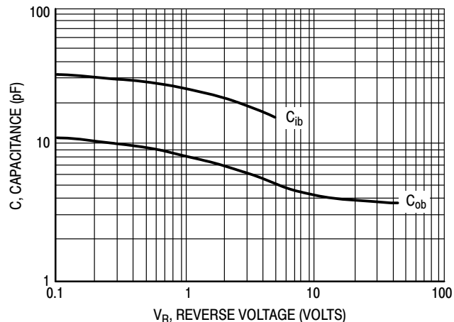
Figure 7. Capacitances
